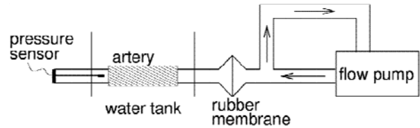
Fig.1. Schematic diagram of the measurement system.
