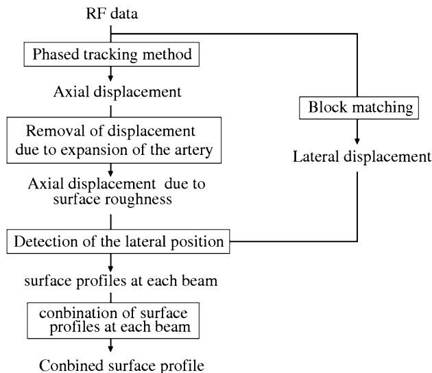
Fig. 2 Procedure for measurement of surface roughness
