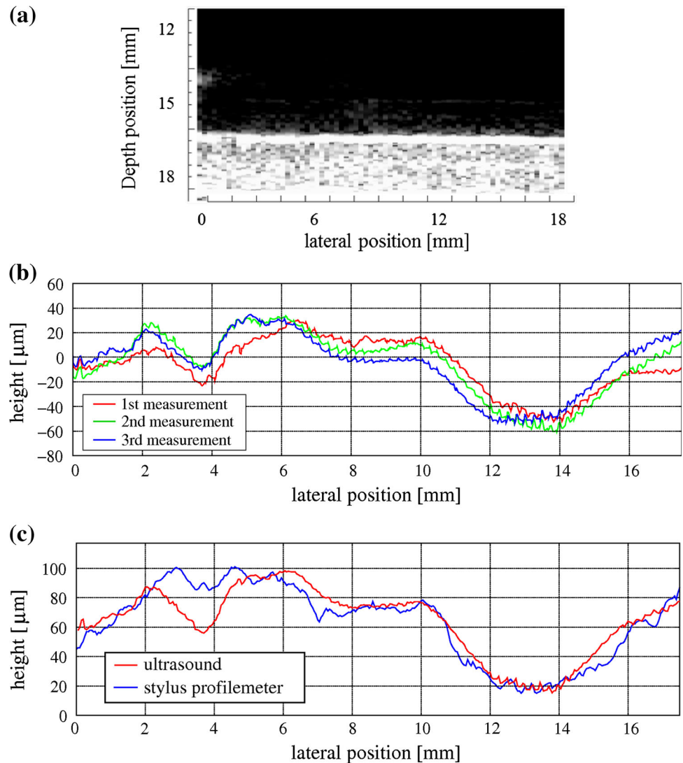
Fig. 6 a B-mode image of the porcine artery. b Surface profiles measured three times by the proposed ultrasonic method. c Averaged surface profile of the porcine artery measured by the proposed method (red line) and stylus profilometer (blue line)
