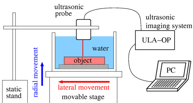
Fig. 5 Illustration of the experimental system. The porcine artery was moved using a movable stage to simulate displacement of carotid arterial wall
