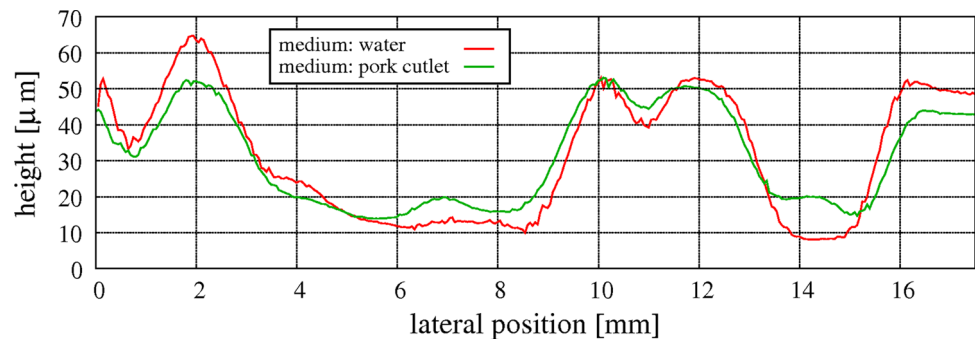
Fig. 7 Surface profiles of the porcine artery measured with (green line) and without (red line) the porcine cutlet between the porcine artery and ultrasonic probe
