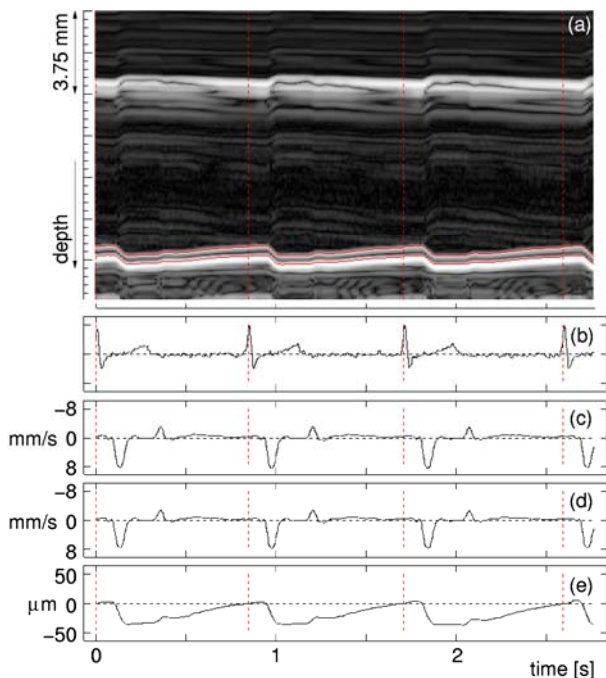
図3. (a) M-mode image of carotid artery of 31-year-old healthy male. (b) Electrocardiogram. (c) Velocity of luminal boundary. (d) Velocity of media-adventitia boundary. (e) Change in thickness of posterior wall.
